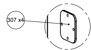
DETAIL D SCALE 1 : 2
